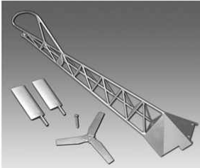
Art.-Nr. / Ord. No. 03 2732 Heckausleger Set Tail truss subassembly
